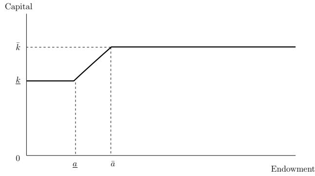
Fig. 1 Optimal Capital Allocation
