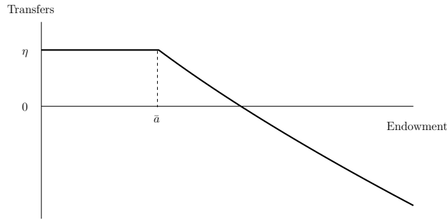
Fig. 1 Optimal Capital Allocation
